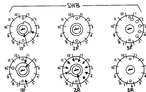
SWITCH POSITION TABLE
