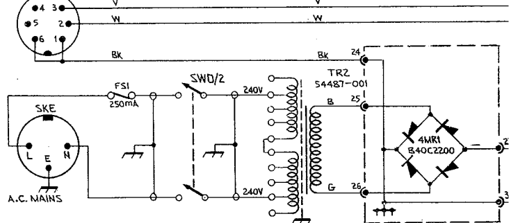
WIRING SIDE OF CONNECTORS
