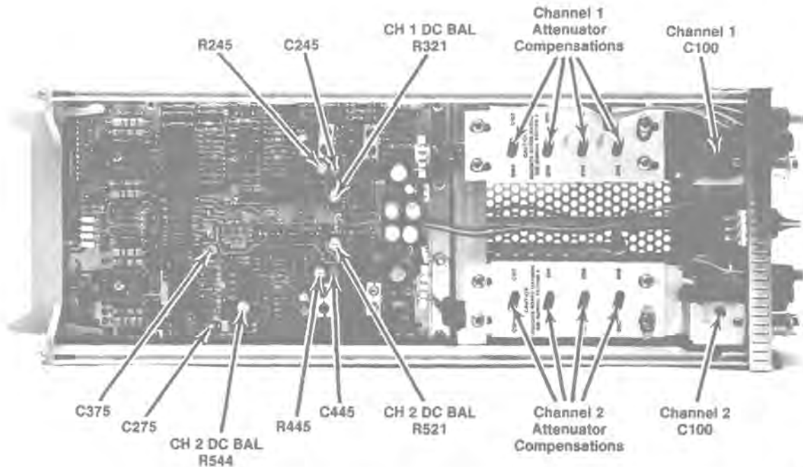
Fig. 4-1. Locations of adjustments used in this procedure.
