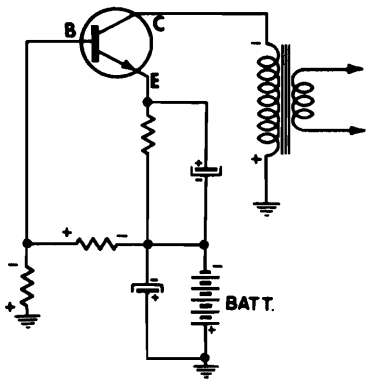
With Positive Battery Terminal Grounded
