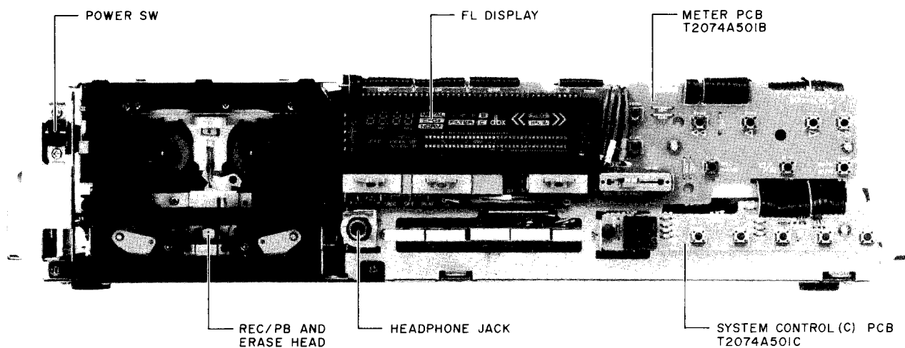
Fig. 4-1 Front View
