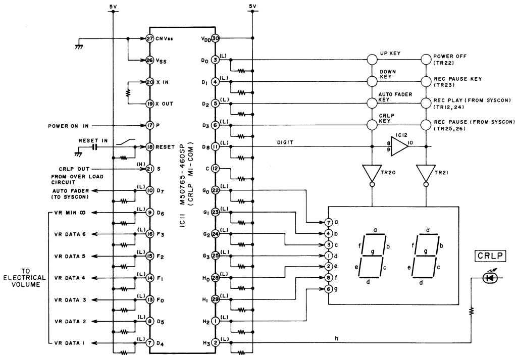
GX-R70 CRLP BLOCK DIAGRAM NO.3-1 850916A(A4)
