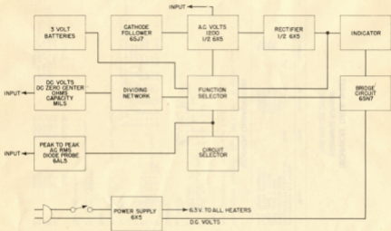
FIGURE 1.2 BASIC DIAGRAM, IN BLOCK FORM, MODEL 209A
