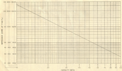
FIGURE 5.1 IMPEDANCE CHART
