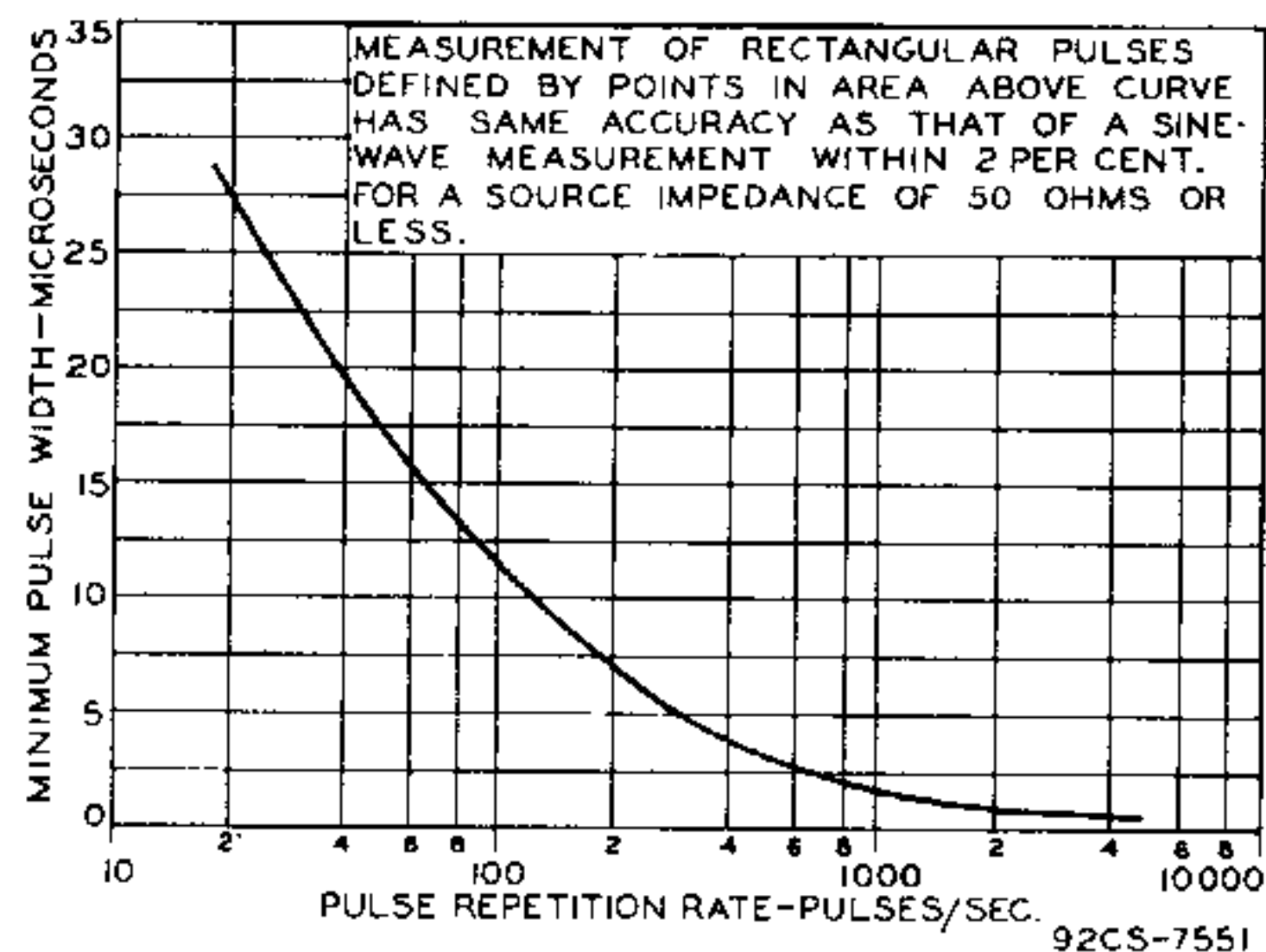
Figure 5. Pulse response capability of the WV-98A
