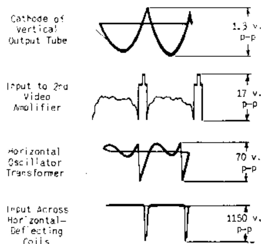
Figure 3. Typical television waveforms
