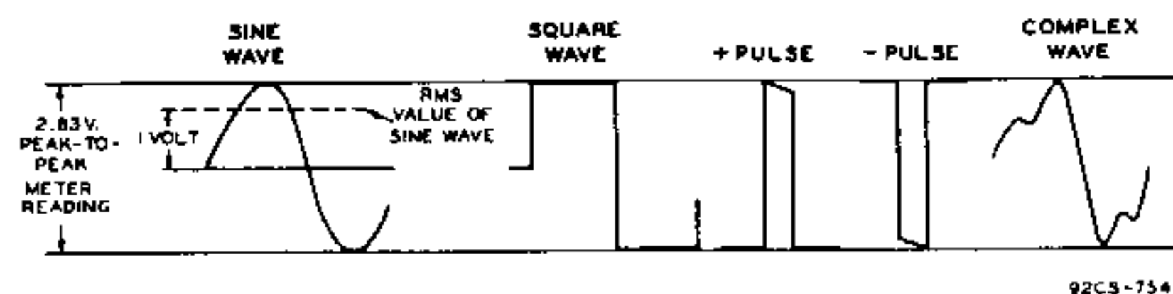
Figure 4. Typical voltage waveforms
