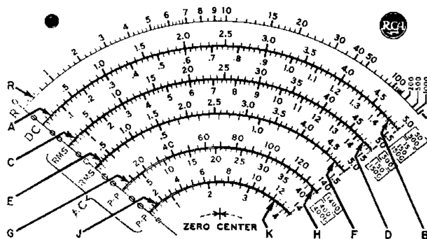
Figure 1. WV-98A meter scales
