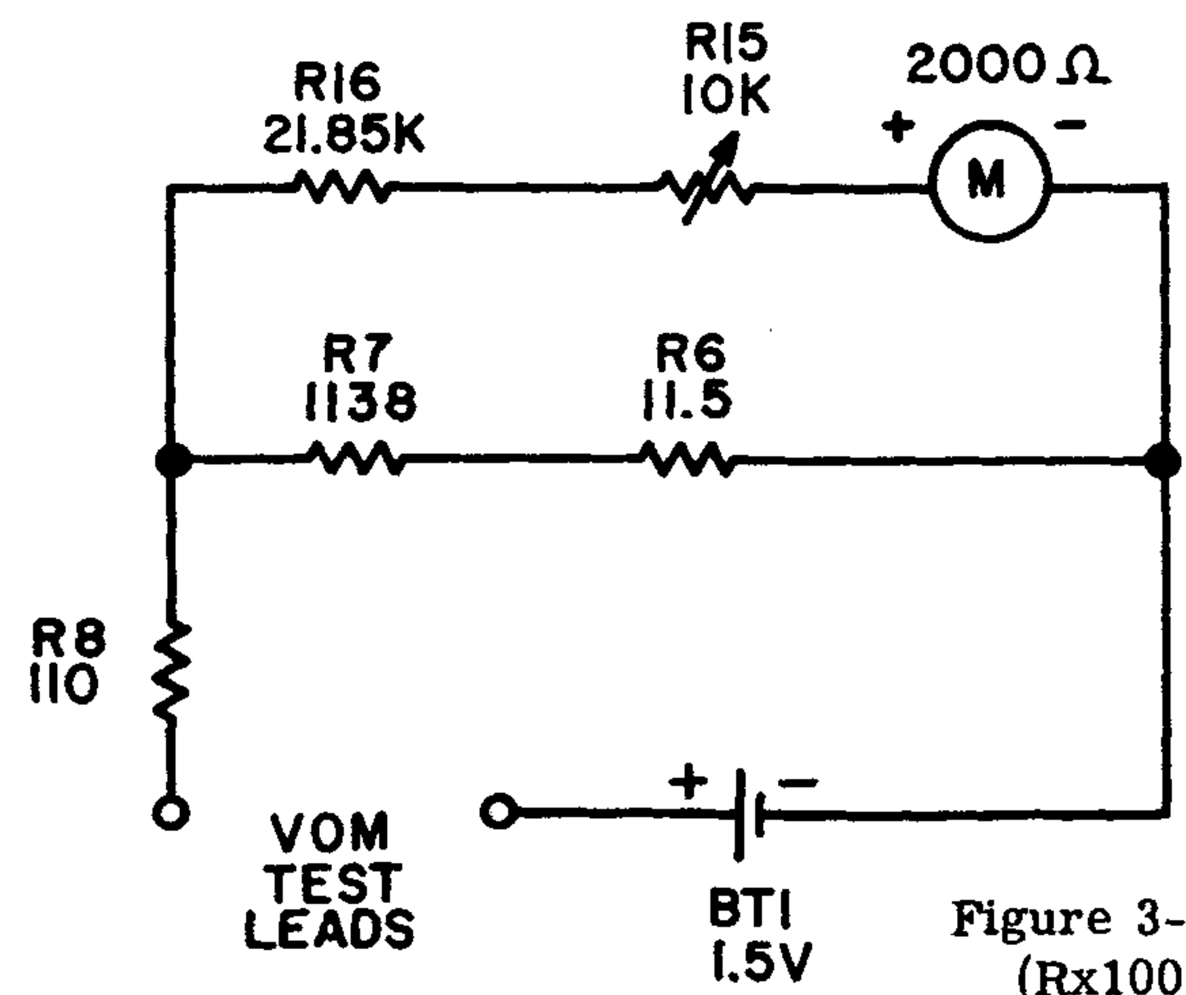
Figure 3-3a. (Rx1)
