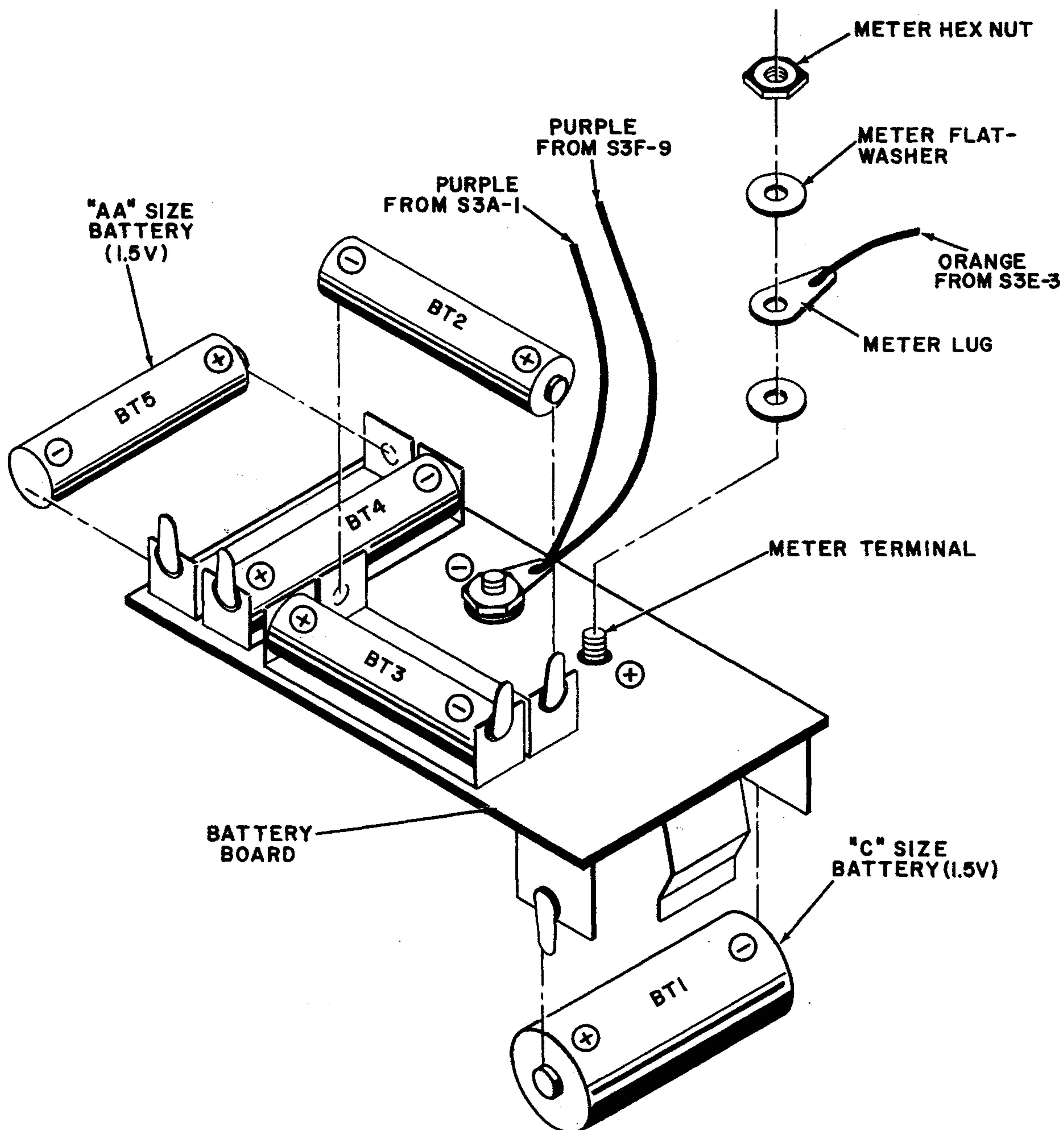
Figure 5-1. Battery Placement
