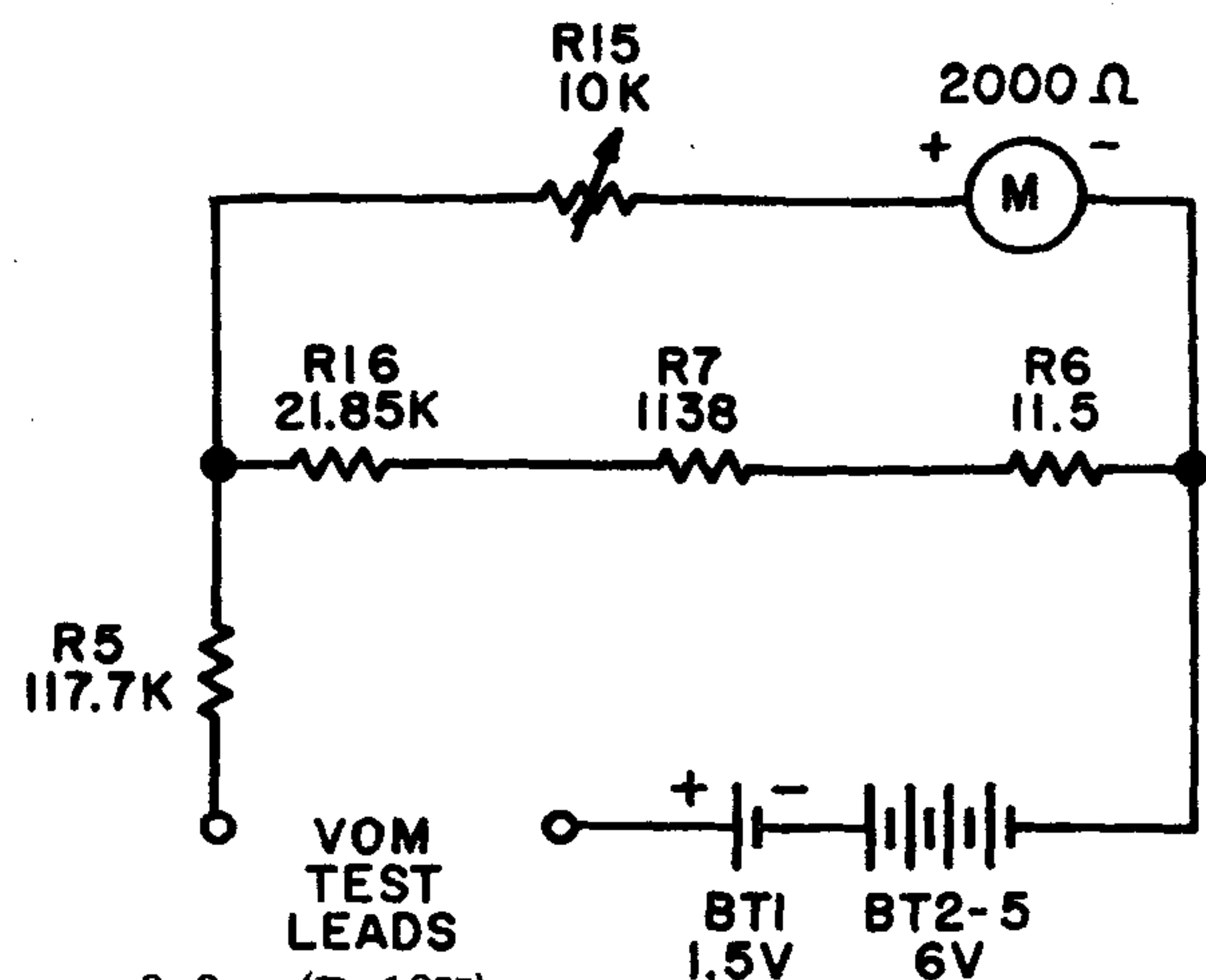
Figure 3-3c. (Rx10K)
