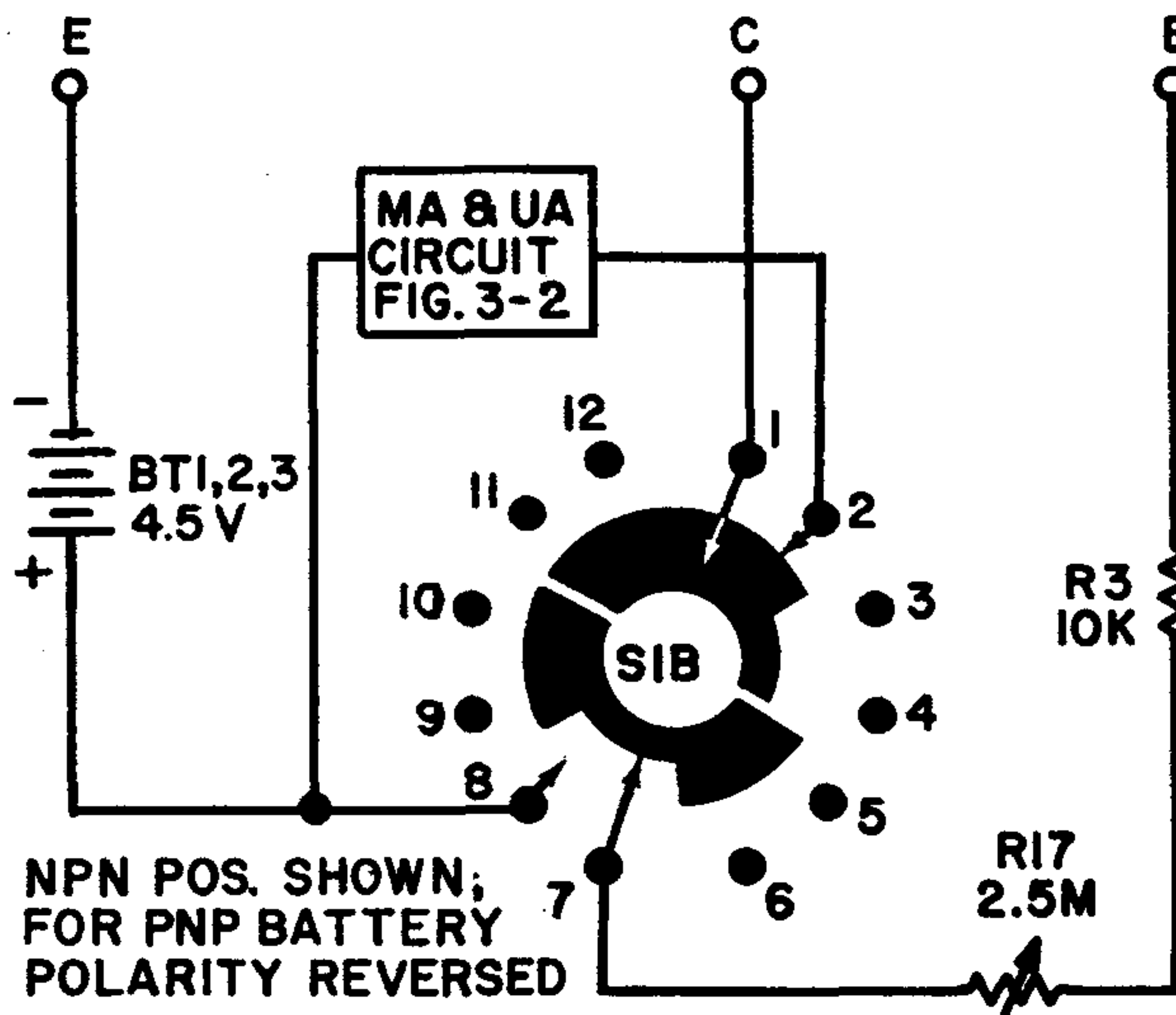
Figure 3-7a. Actual Circuit Switching
