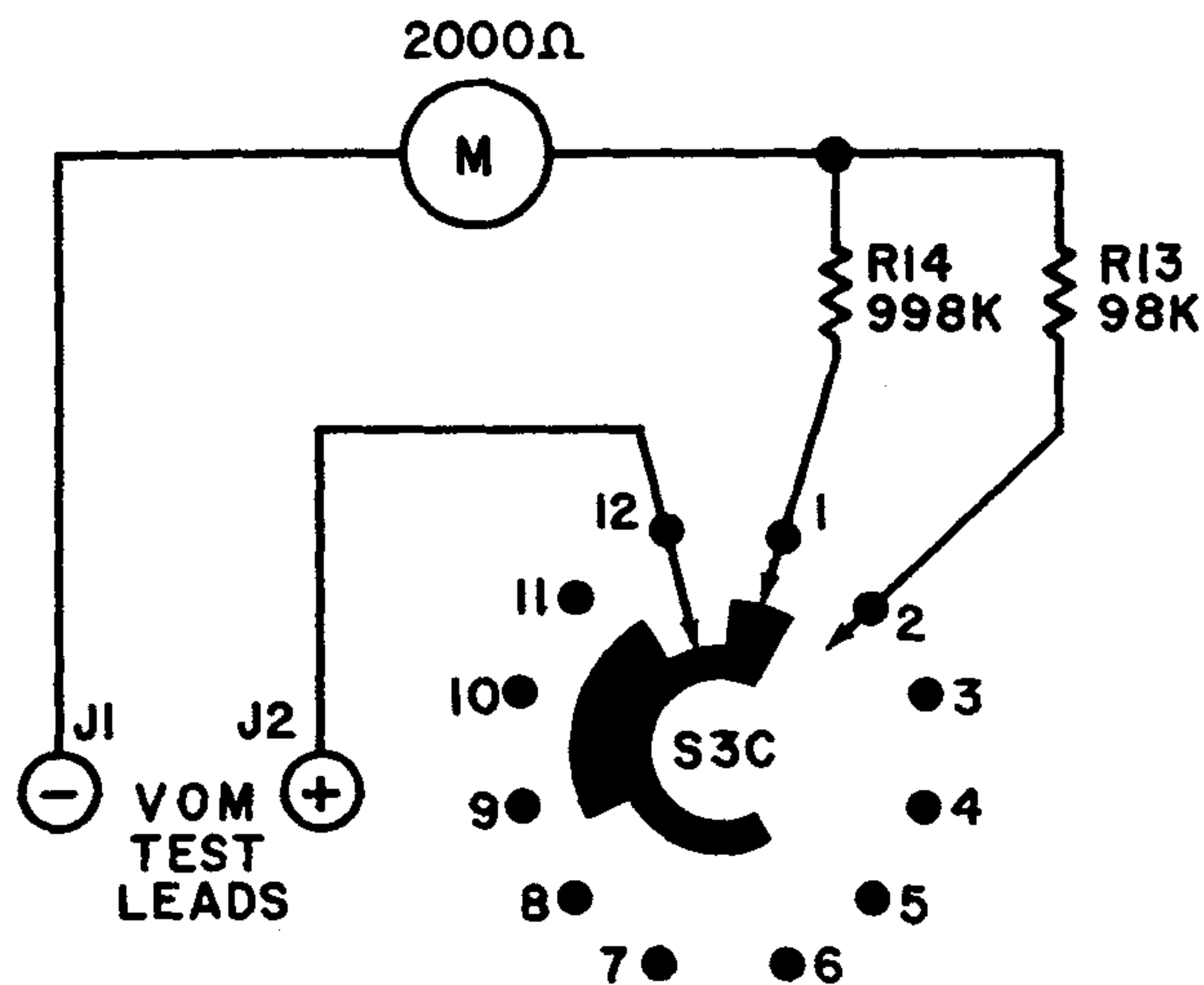
Figure 3-1. Voltmeter Circuit
