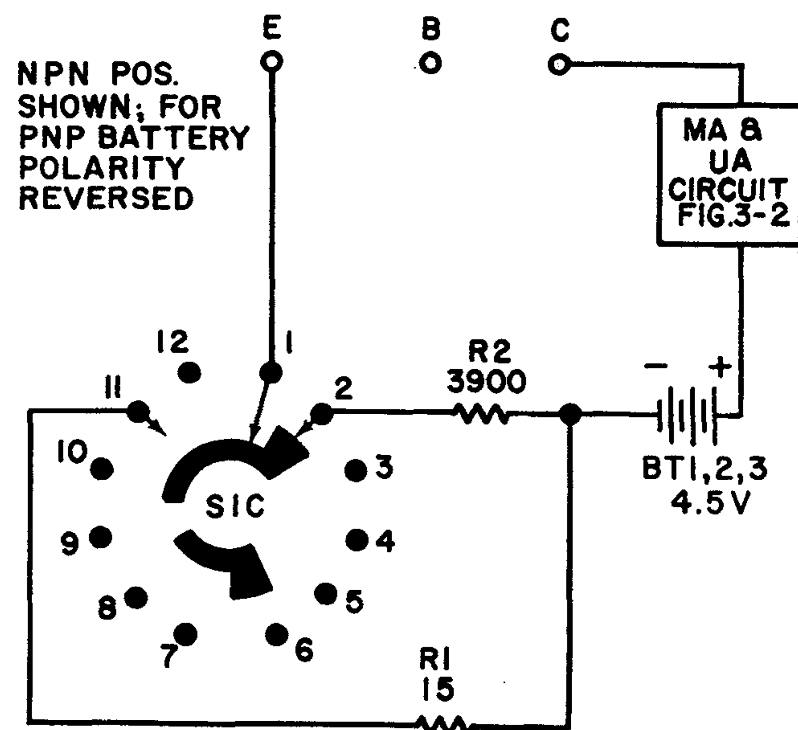
Figure 3-6. ICEO Test Circuit
