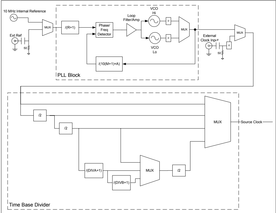
Figure 6: DBS2050A Clock Diagram
