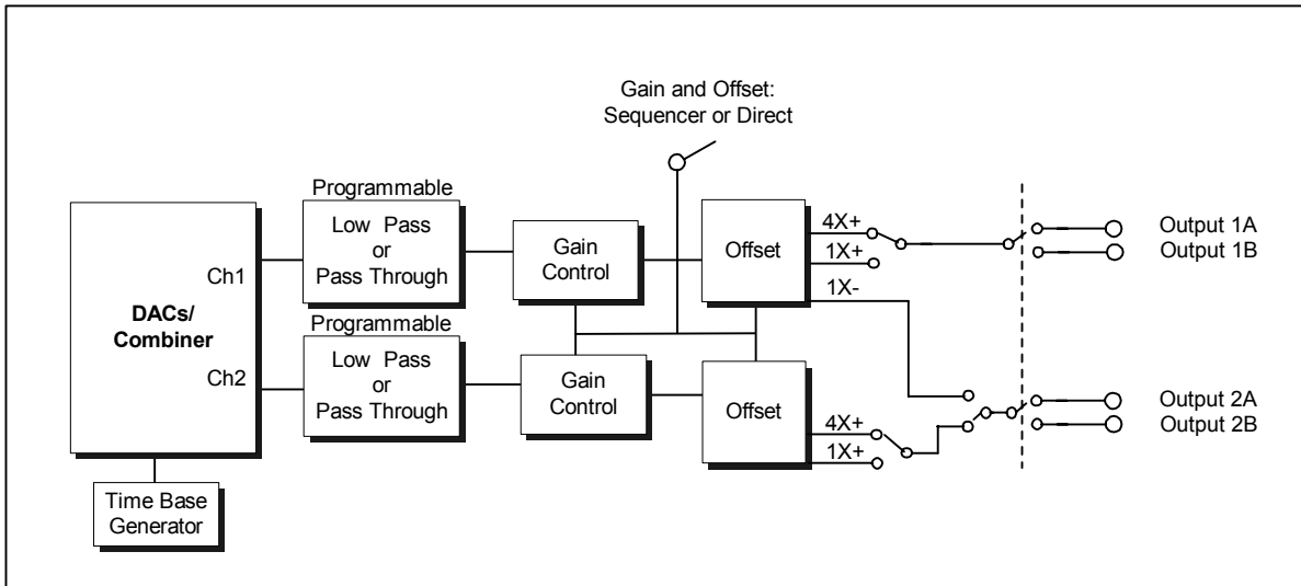
Figure 5: Channel Mode Block Diagram
