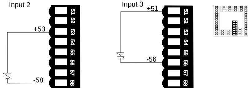
Figure 12.5b — 0-20mA or 4-20mA Process
