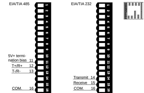
Figure 12.10a — EIA/TIA 485 and EIA/TIA 232 Communications
