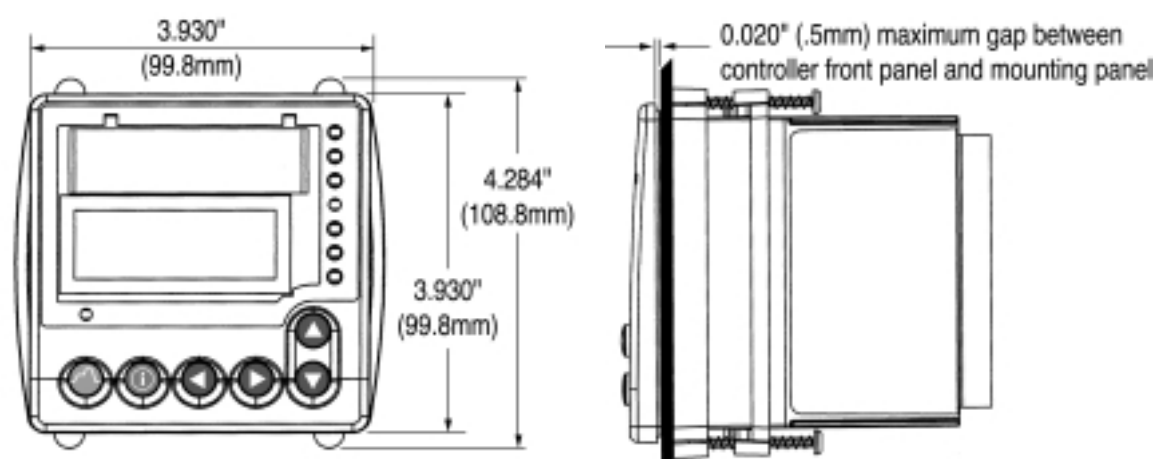
Figure 11.1a — Front View Dimensions and Gasket Gap Dimension.
