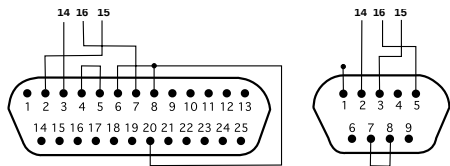
Figure 12.10c — EIA/TIA-232 Connections
