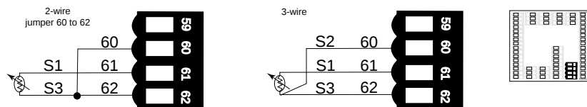
Figure 12.3c — 0-5V \rightleftharpoons , 1-5V \rightleftharpoons or 0-10V \rightleftharpoons (dc) Process
