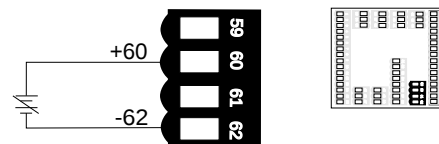
Figure 12.3e — 0 to 50mV
