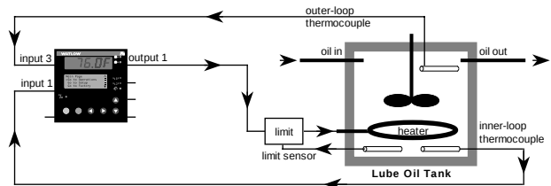
Figure 6.11c — Cascade Example
