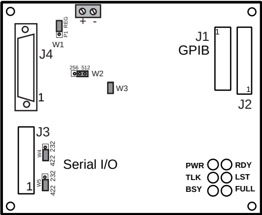
Figure 2-14 4809 W4 and W5 Jumpers set to RS-422 Position
