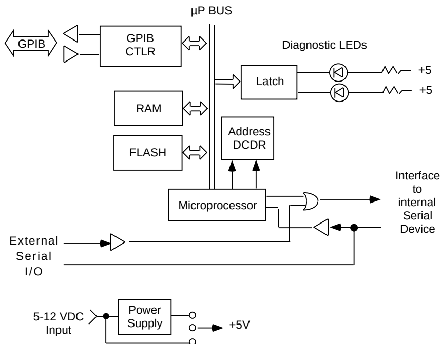
Figure 4-2 4819 Block Diagram
