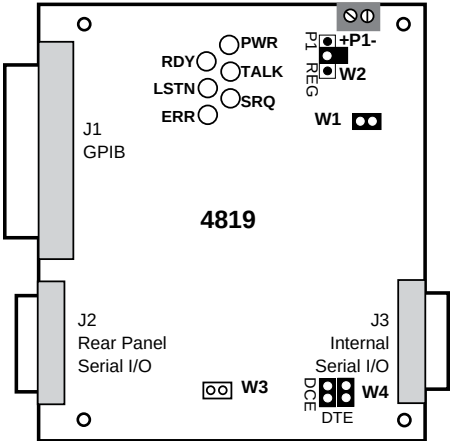
Figure 2-15 4819 Jumper Locations
