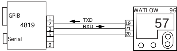
Figure 2-10 4819 RS-232 Connections to a Watlow 96
