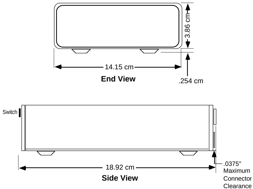
Figure 1-2 4899 Outline Dimensions
