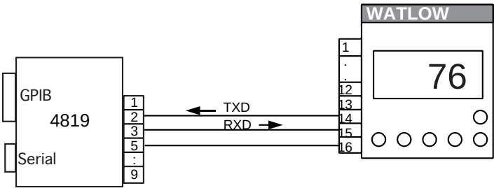
Figure 2-9 4819 RS-232 Connections to a Watlow F4
