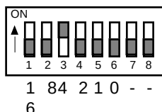
Figure 2-5 Address Switch Rocker Assignments
