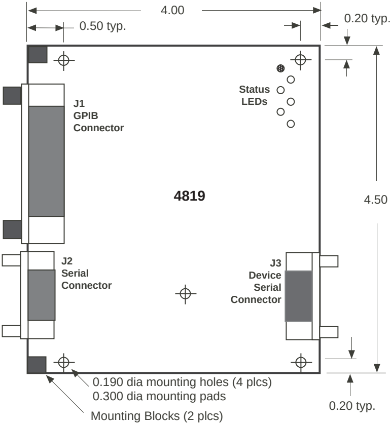
Figure 1-4 4819 Outline Dimensions
