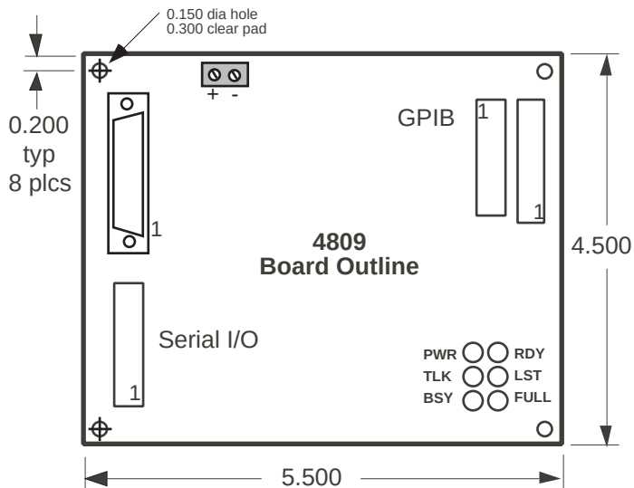
Figure 1-3 4809 Outline Dimensions
