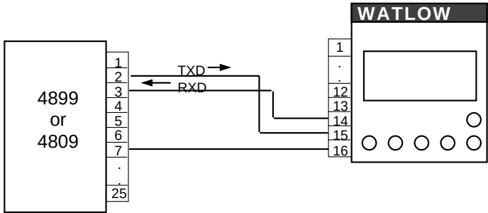
Figure 2-8 4899/4809 RS-232 Connections to a Watlow F4
