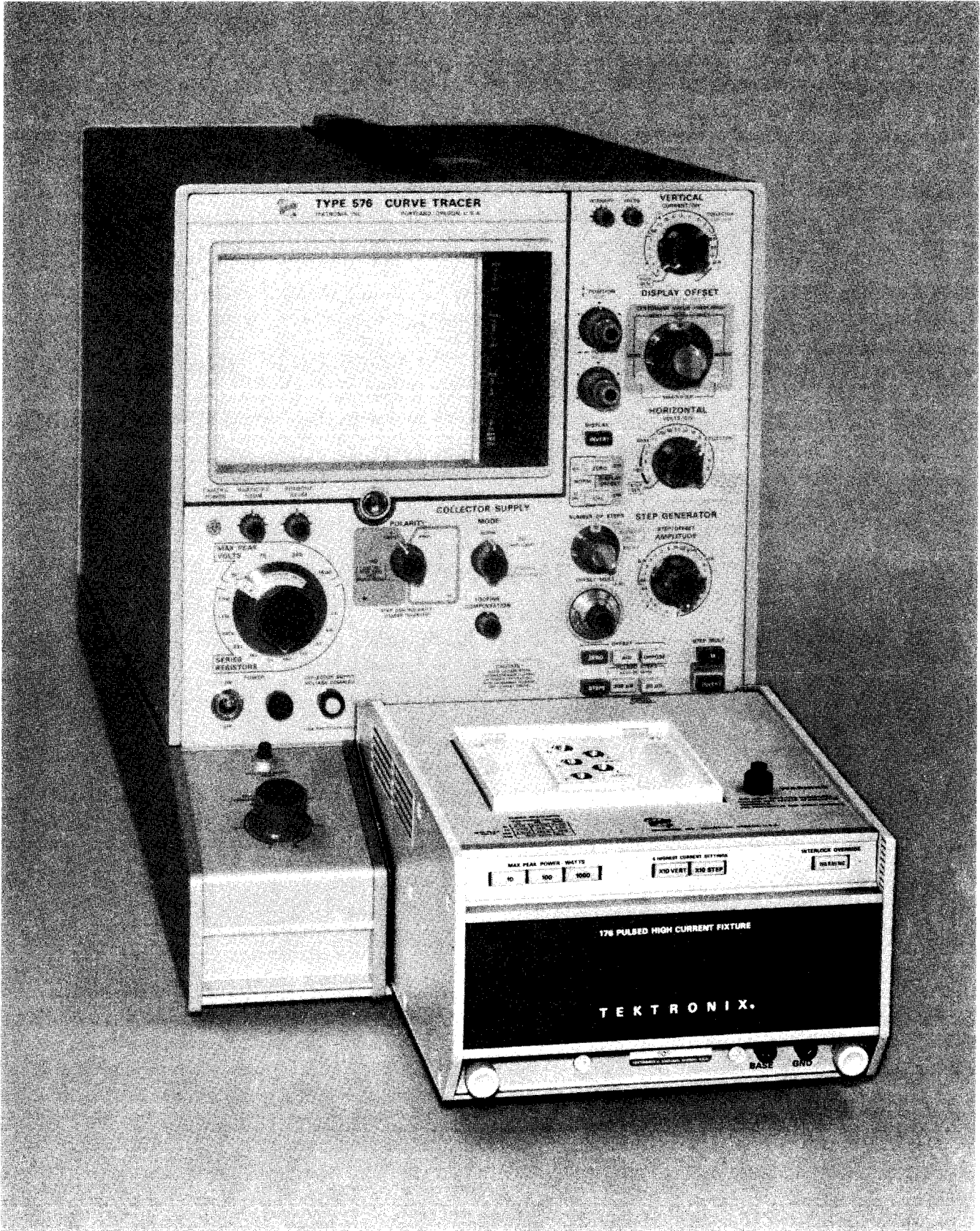
Fig. 1-1. 176 High-Current Fixture.
