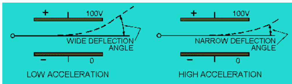
Figure 6-6.—Beam acceleration.
