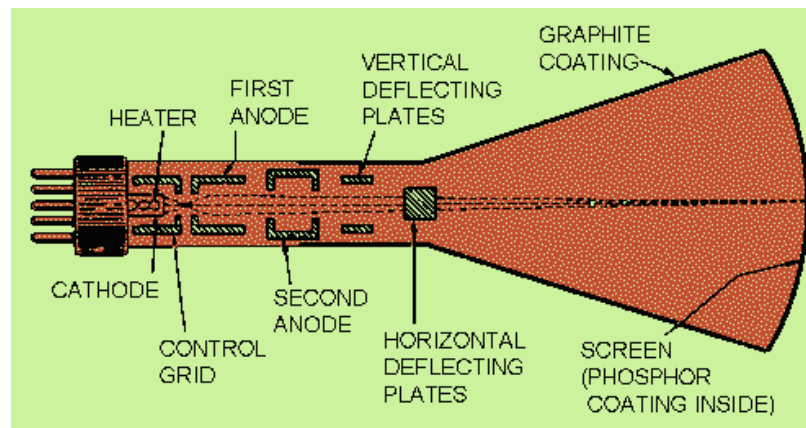
Figure 6-1.—Construction of a CRT.
