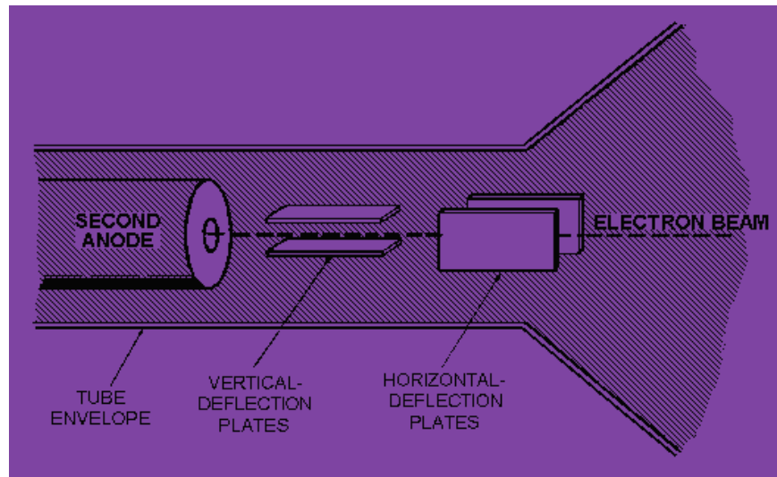
Figure 6-7.—Deflection plate arrangement.
