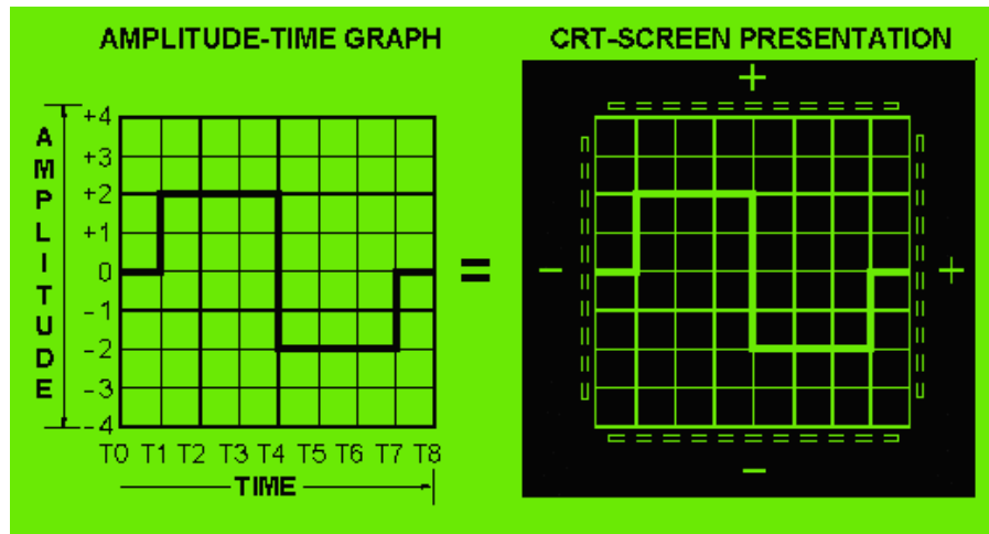
Figure 6-10.—Amplitude versus time.
