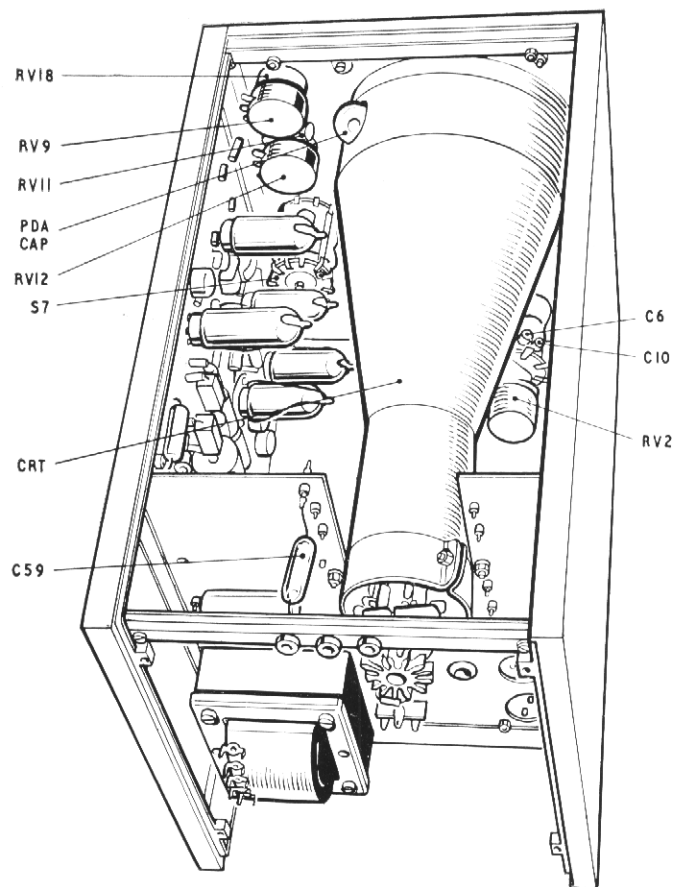
Fig. 3 Component Location—Top View
