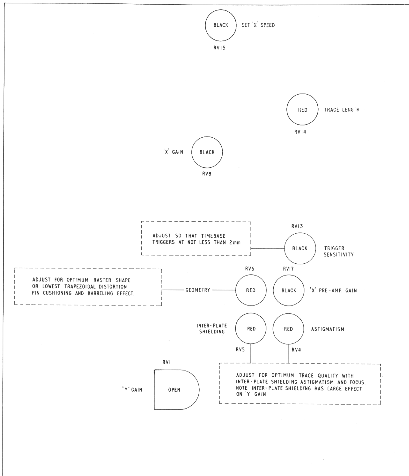
Fig. 6 Functions of Preset Controls on Printed Circuit Board
