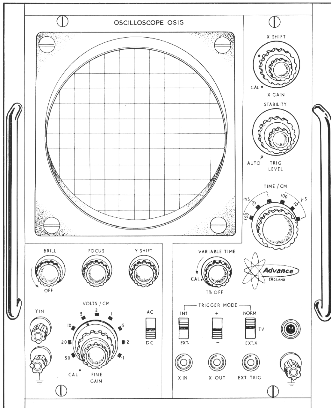
Fig. 1 Front Panel Layout
